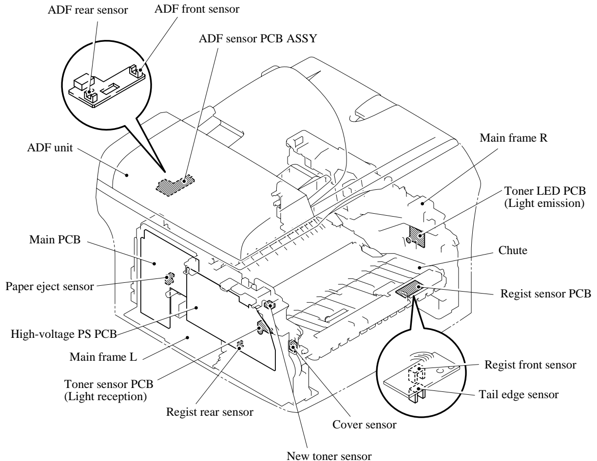
Sensors and Actuators Locations
