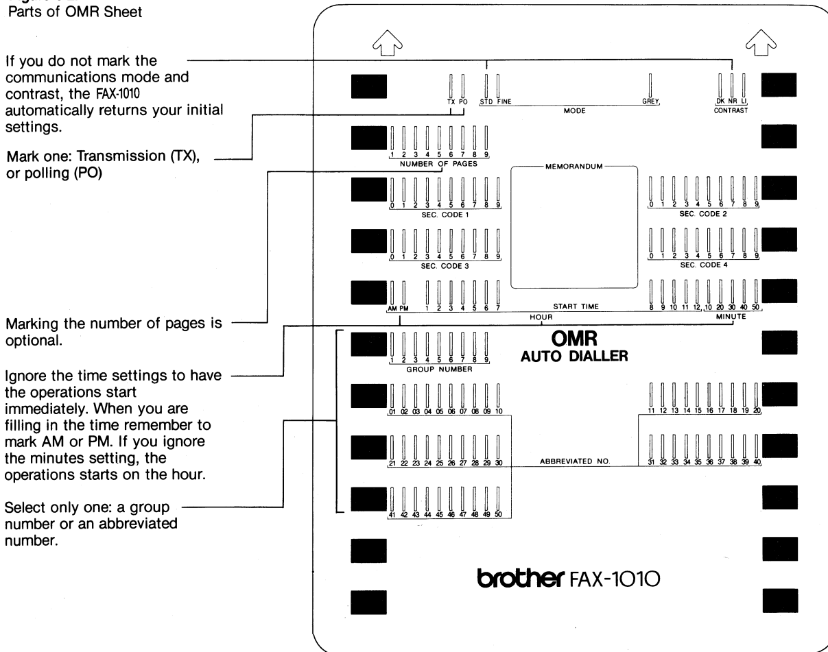
Figure 3-2. Parts of OMR Sheet
