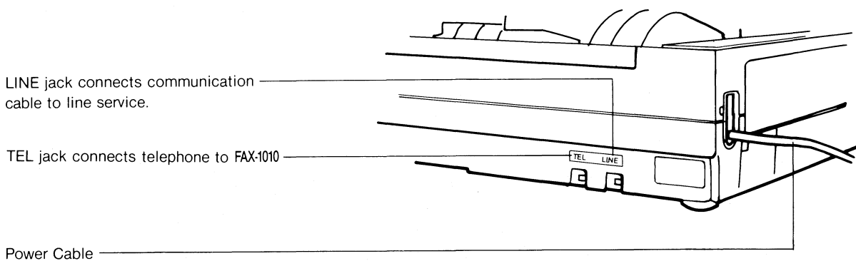
Figure 1-3. Side View
