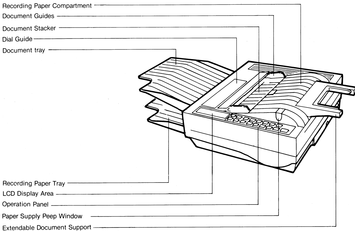
Figure 1-1. Front View
