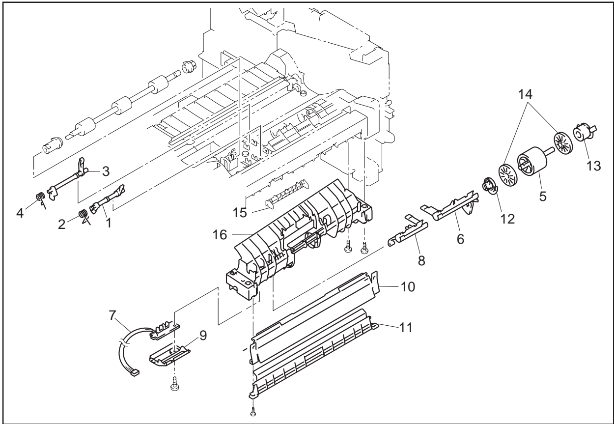
MODEL HL-5030/5040/5050/5070N/5050LT US 84U-Z41/Z42/Z43/Z44/Z46-040
